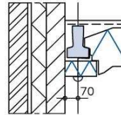
DETAIL - KOPLEGGING ZONDER RANDKIST
